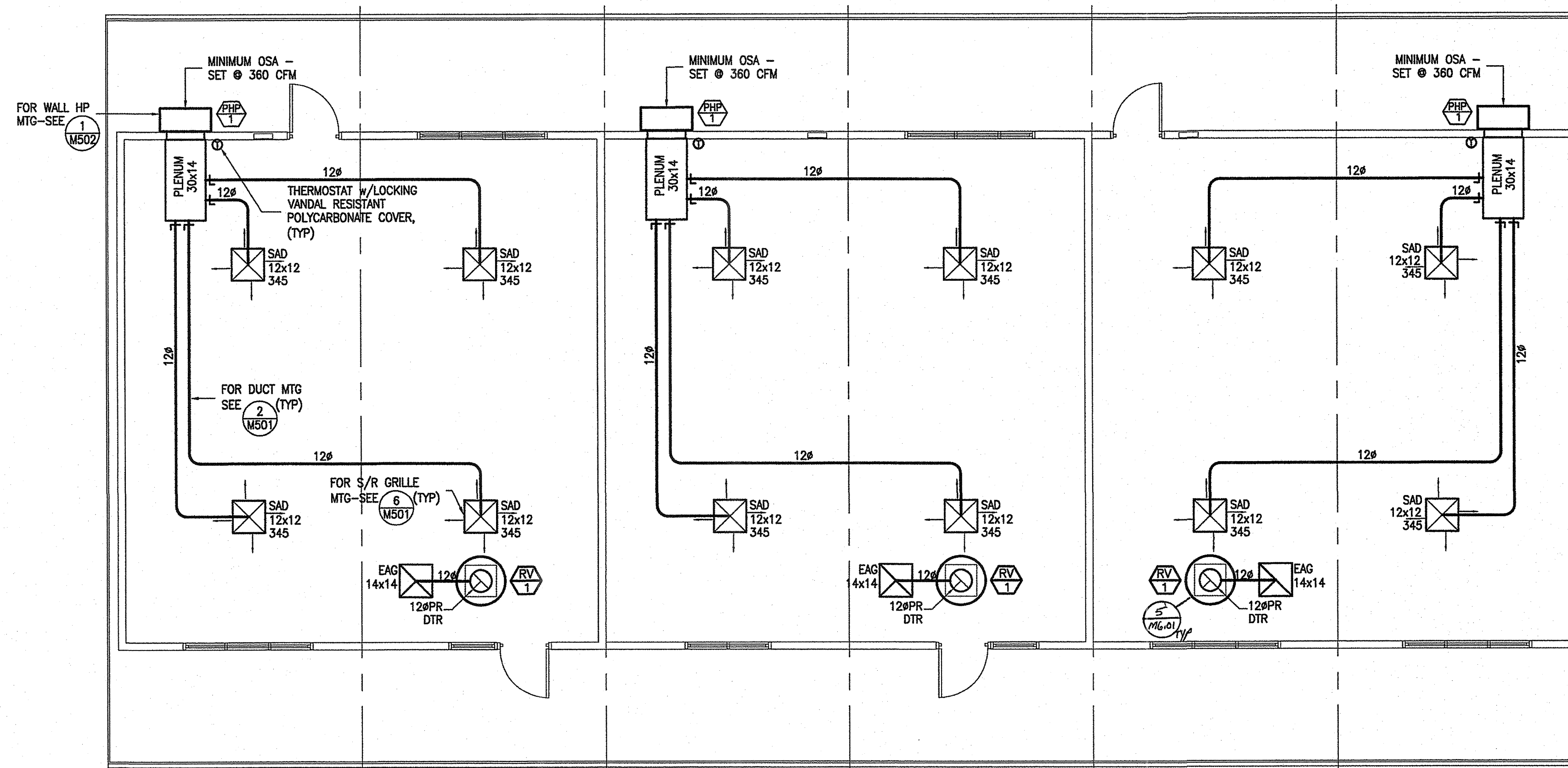
2 SOG 32 - MECHANICAL PLAN - 6M (ALTERNATE 'B')
