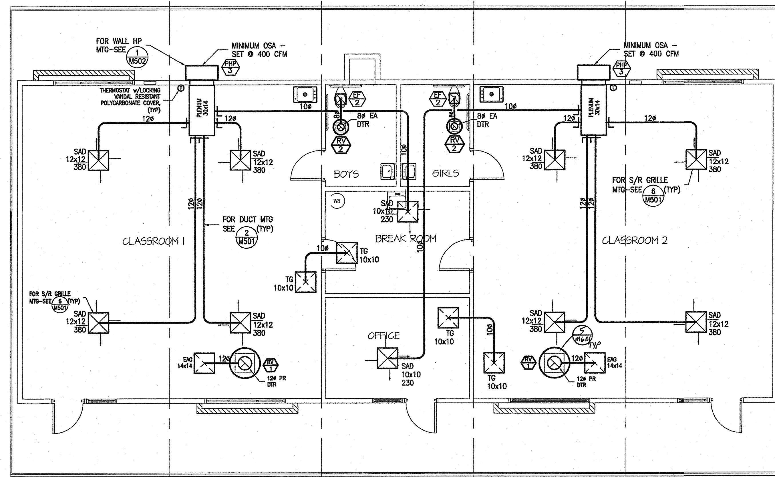
1 SOG 32 - MECHANICAL PLAN - 5M RESTROOM OPTION (ALTERNATE 'B')
